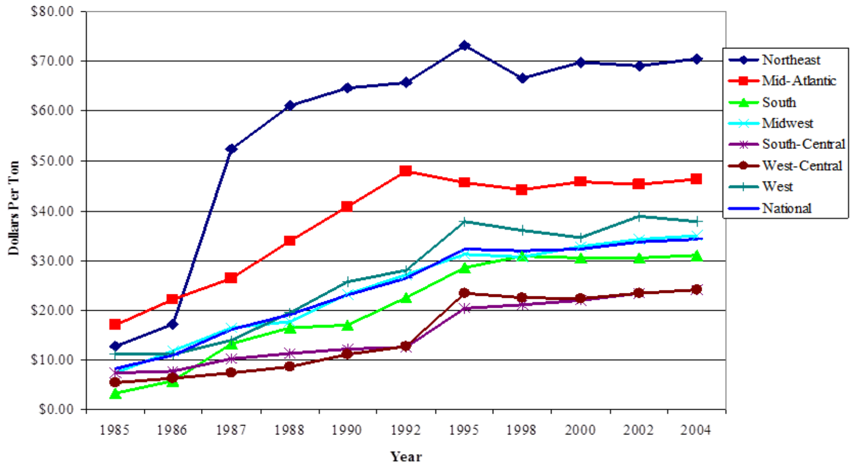
Figure 6 Tipping Fees
