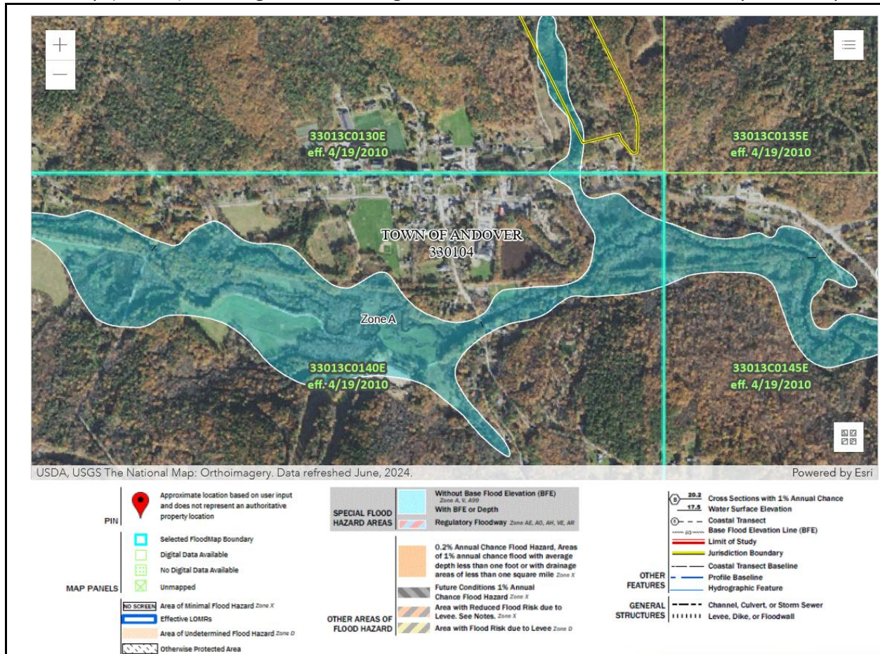
FEMA map (DFIRM) showing Andover Village with the Blackwater River and 100-year-floodplain
