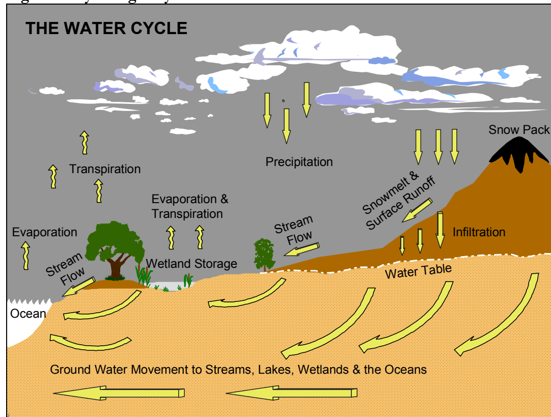
Figure 1. Hydrologic Cycle
