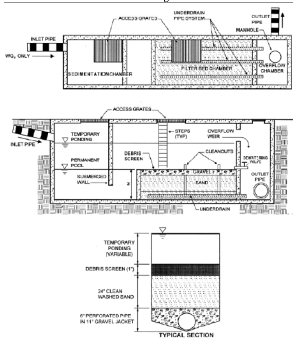
Schematic of an underground sand filter
