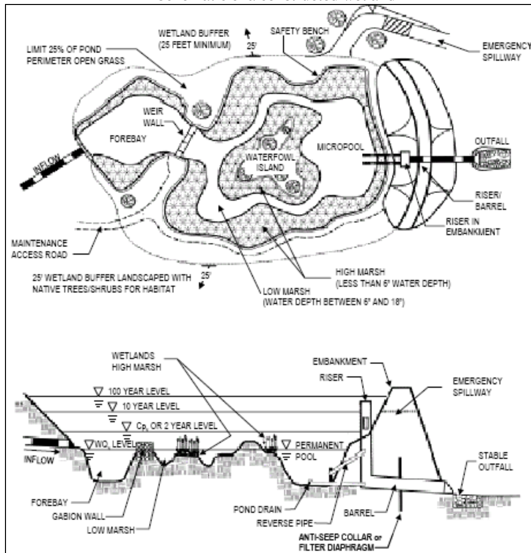
Schematic of a constructed wetland
