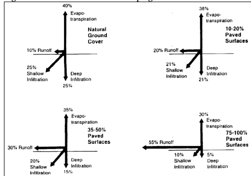
Figure 6. Infiltration Rates in Developing Conditions
