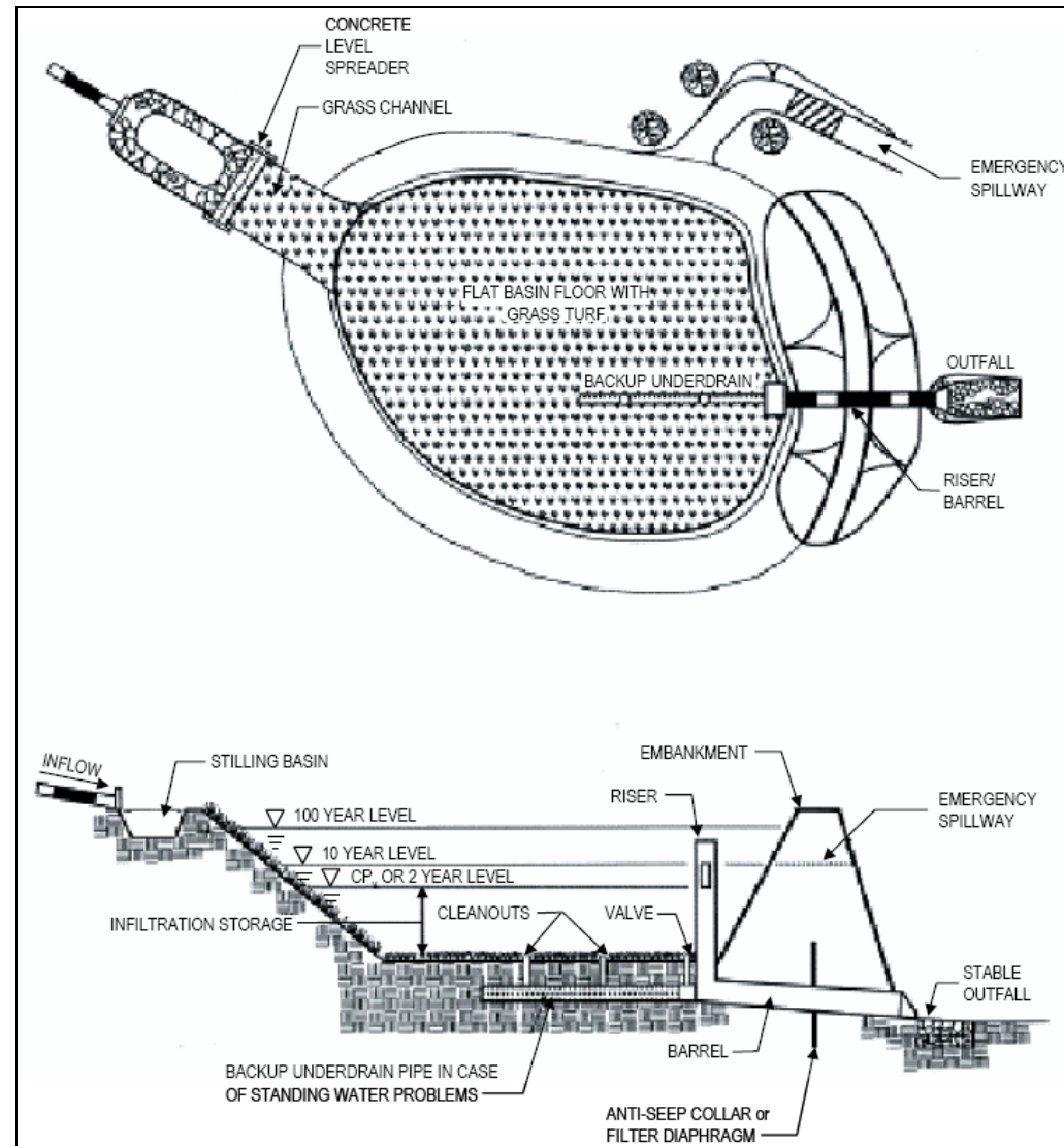
Schematic of an Infiltration Basin
