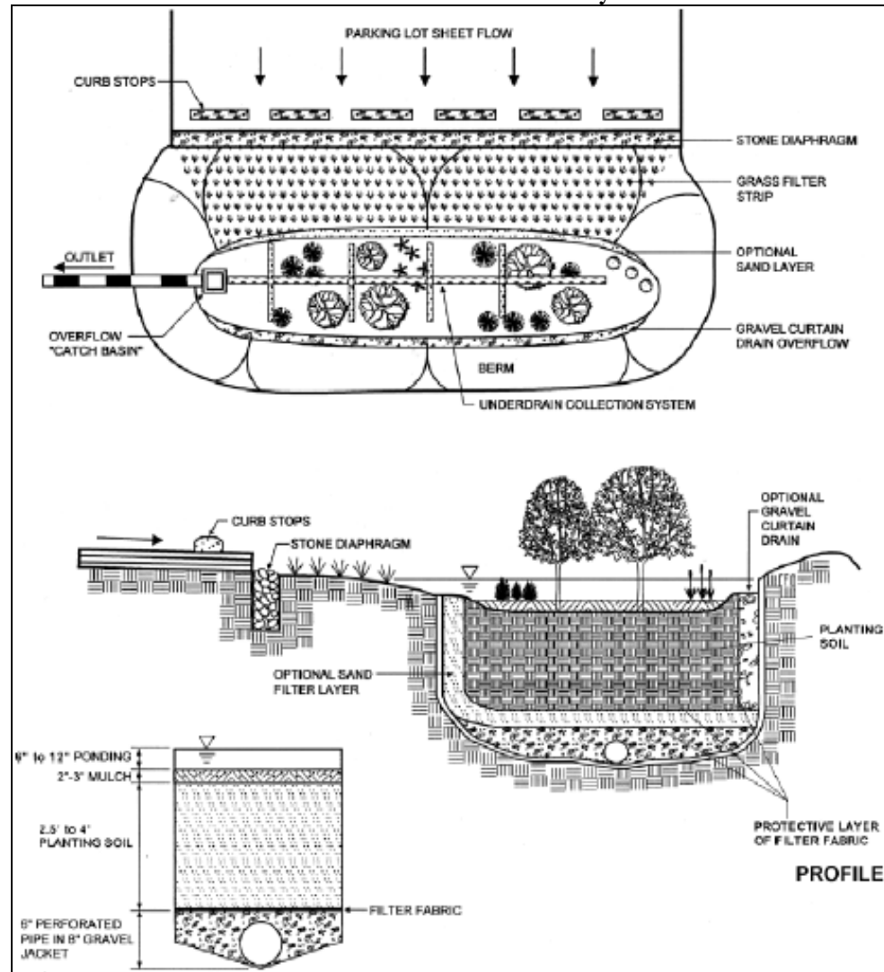
Schematic of a Bioretention system
