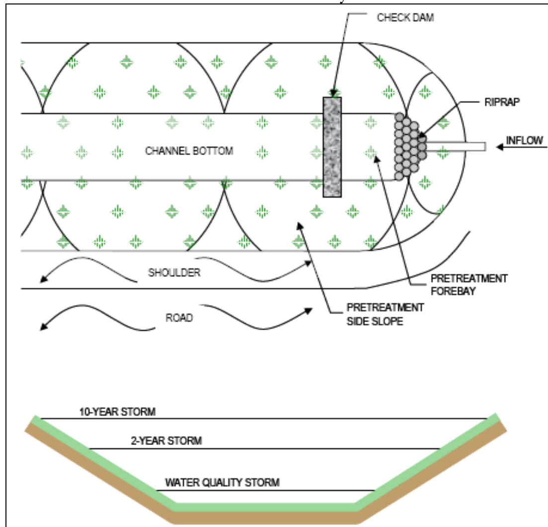
Schematic of a dry swale
