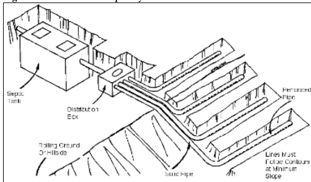
Figure 16. Conventional Septic System
