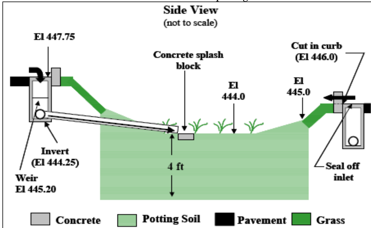
Schematic of a Bioretention parking lot island
