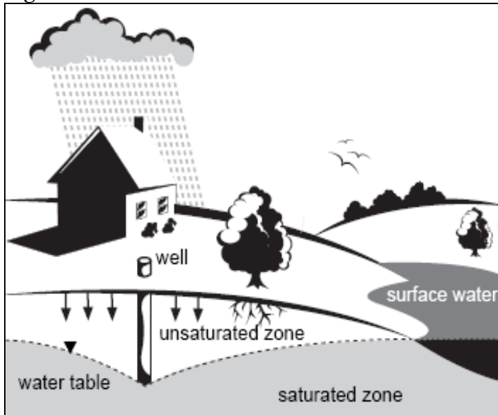
Figure 2. Saturated Zone
