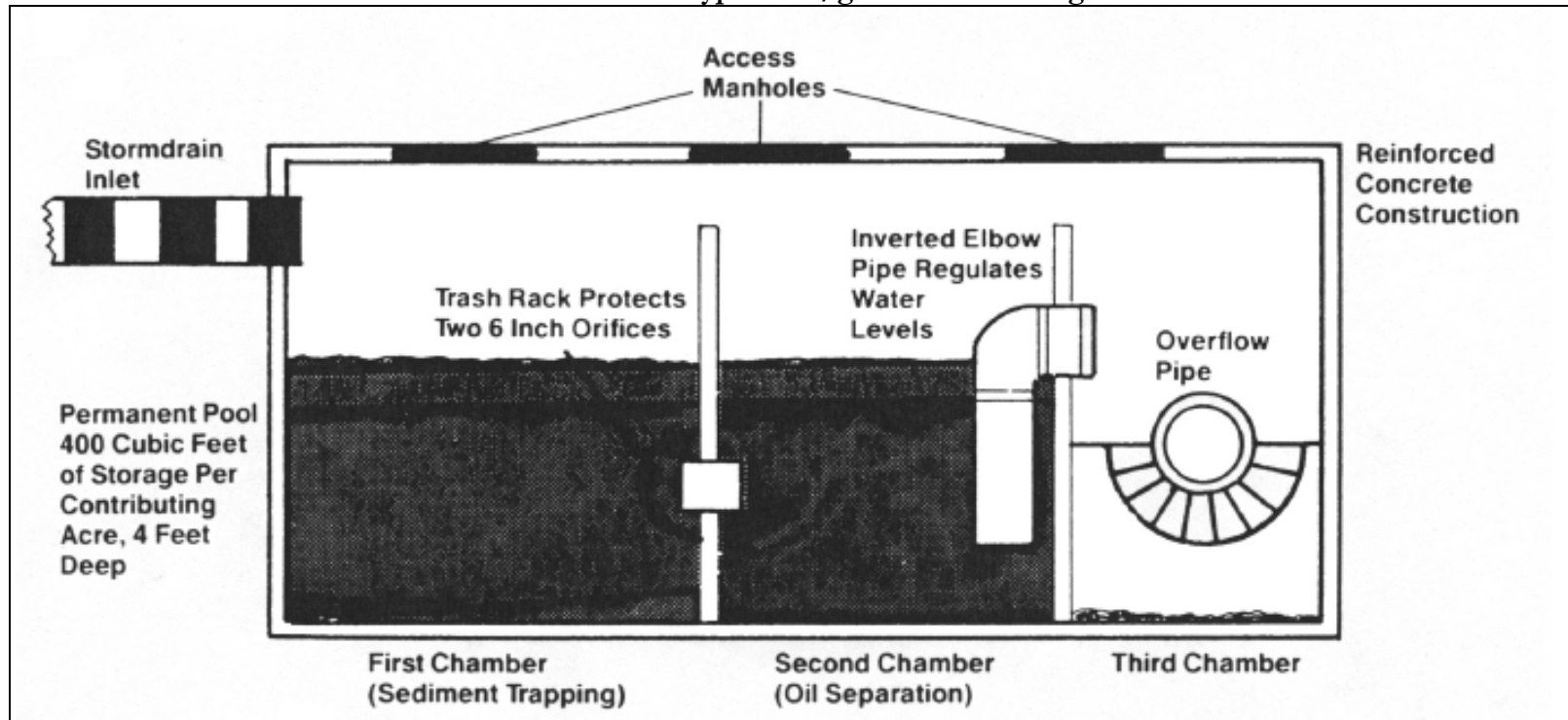
Schematic of a typical oil/grit chamber design
