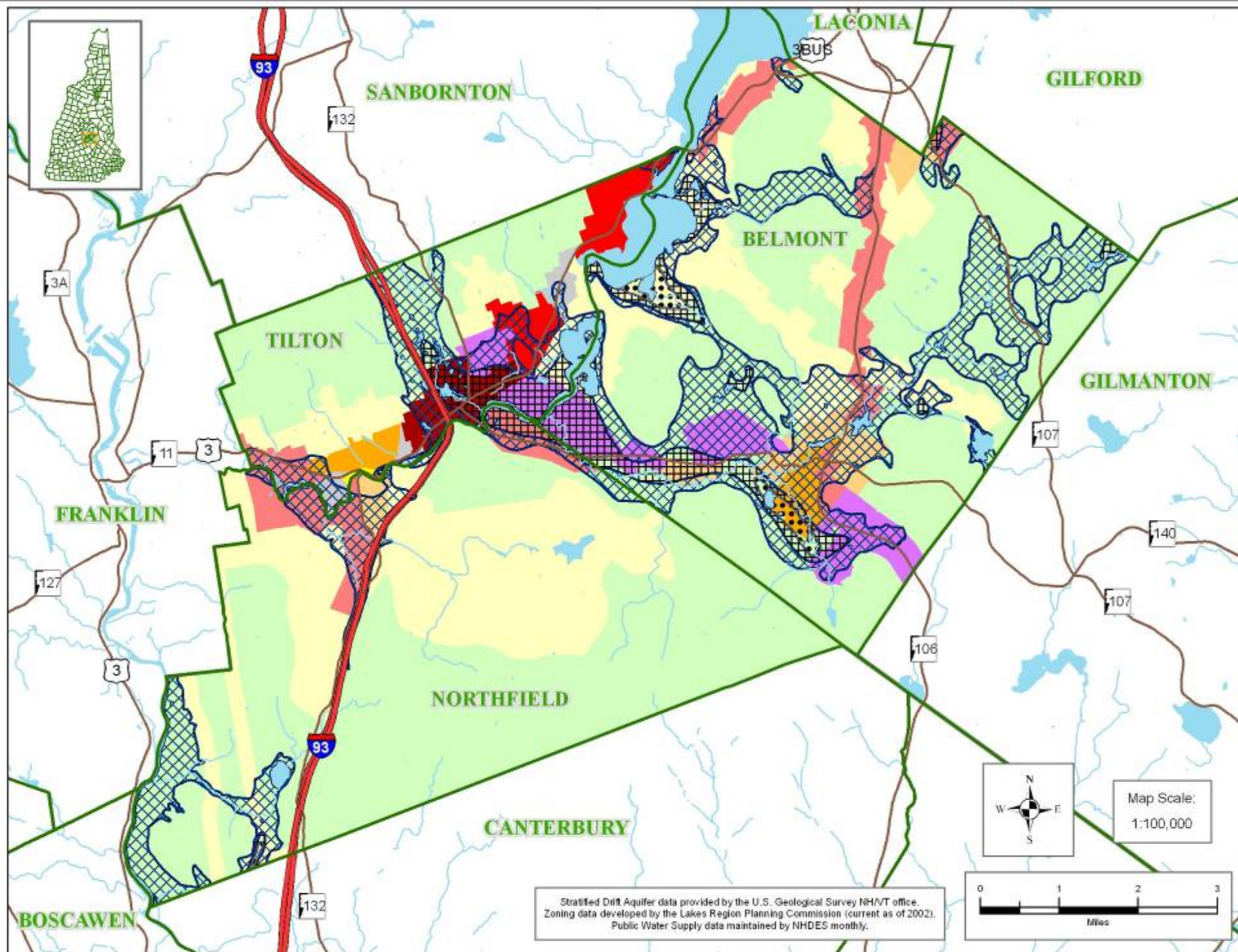
Figure 4: Stratified Drift Aquifer and Zoning
