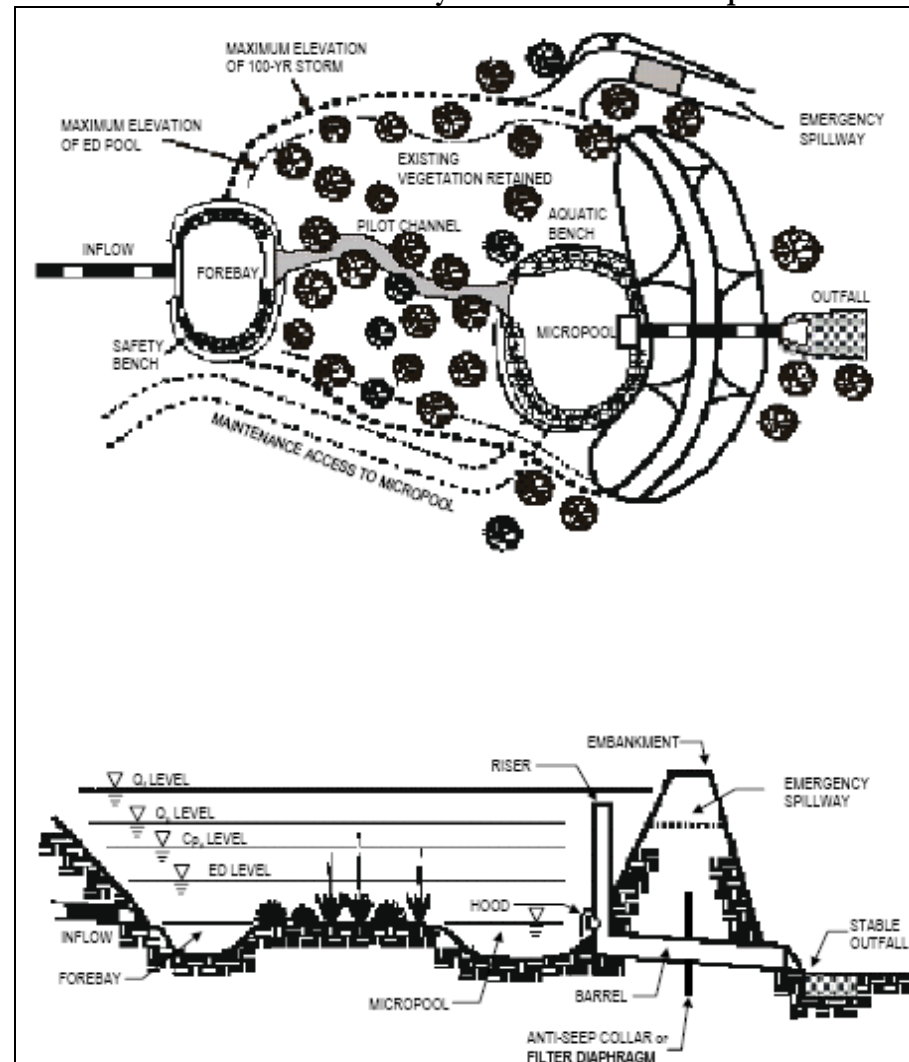
Schematic of a dry extended detention pond
