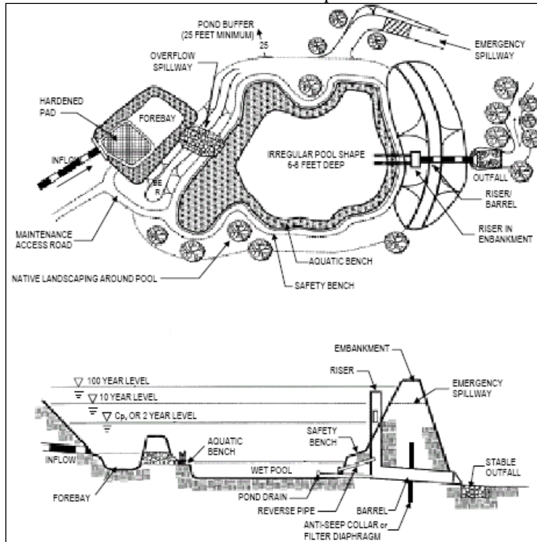
Schematic of a wet pond
