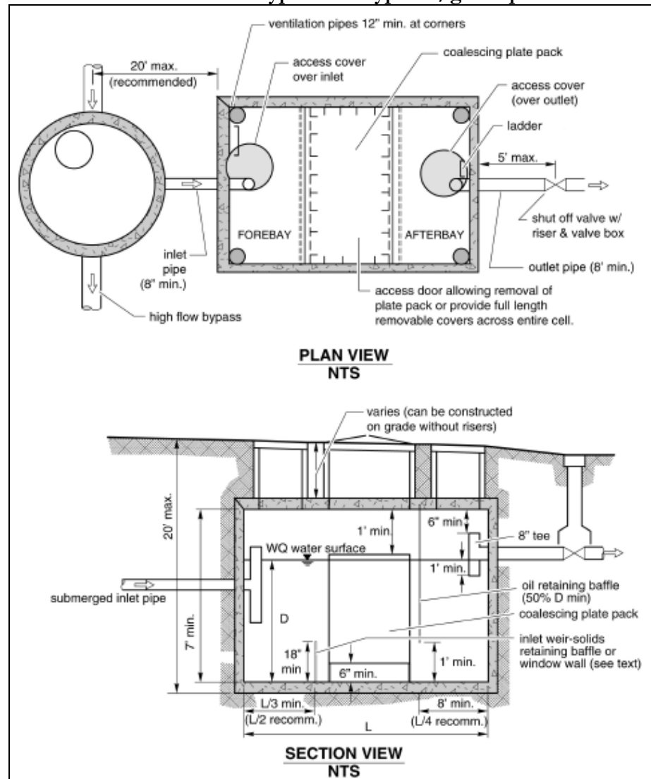
Schematic of a typical CP-type oil/grit separator
