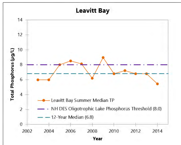
Figure 3.1. Trends for total phosphorus (TP) values (in µg/L or parts per billion (ppb)) in the study lakes from 2003-2014. Also shown is the twelve-year median for each lake (blue dashed line), NH State TP thresholds (purple dashed line) for oligotrophic (Ossipee Lake and Broad, Leavitt, and Berry Bays) and mesotrophic (Danforth Ponds). Mann-Kendall tests revealed no significant trends in TP concentrations over the time period.
